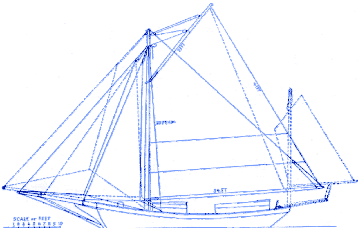
The solid lines represent the sail-plan of the Spray on starting for the long voyage. With it she crossed the Atlantic to Gibraltar, and then crossed again southwest to Brazil. In South American waters the bowsprit and boom were shortened and the jigger-sail added to form the yawl-rig with which the rest of the trip was made, the sail-plan of which is indicated by the dotted lines. The extreme sail forward is a flying jib occasionally used, set to a bamboo stick fastened to the bowsprit. The manner of setting and bracing the jigger-mast is not indicated in this drawing, but may be partly observed in the plans on pages 287 and 288.
